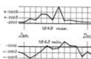
Annual Inequality of Diurnal Range of Horizontal Force, as referred to the Mean Inequality.
