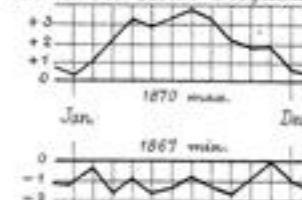
Annual Inequality of Diurnal Range of Declination, as referred to the Mean Inequality.
